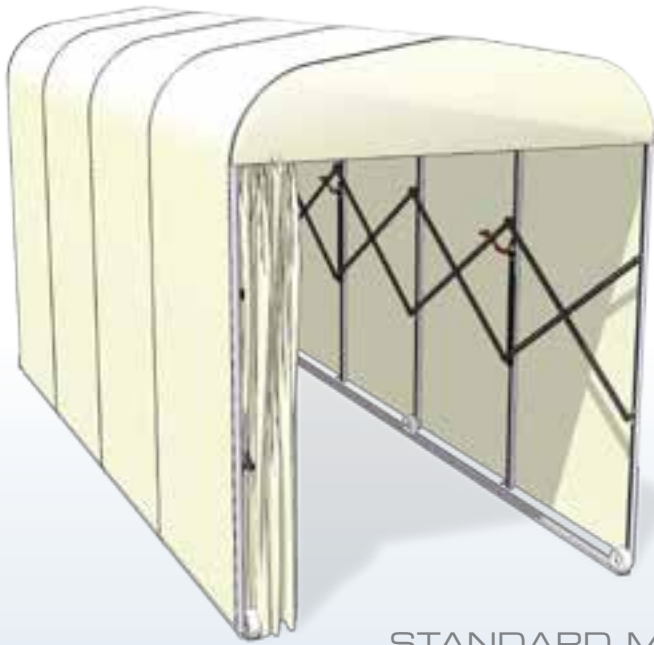
STANDARD MODEL
